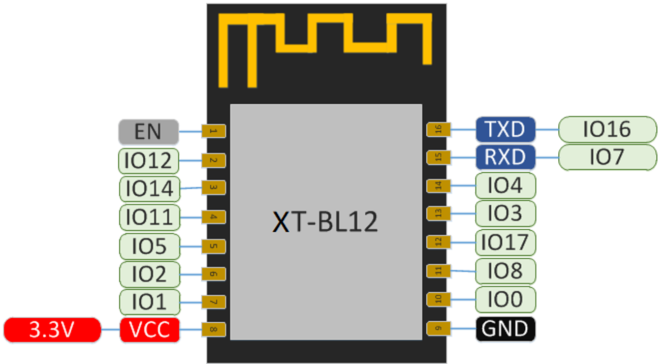
Fig.2.1 XT-BL12 Pin Definition
