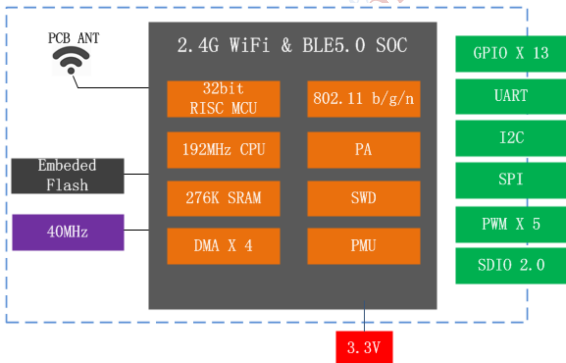
Fig.1.1 XT-BL12 Module Structure
