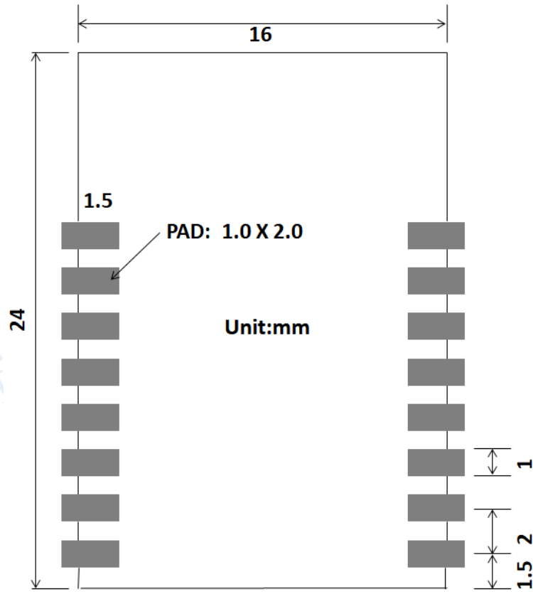
Fig.3.3 PCB Layout for XT-BL12
