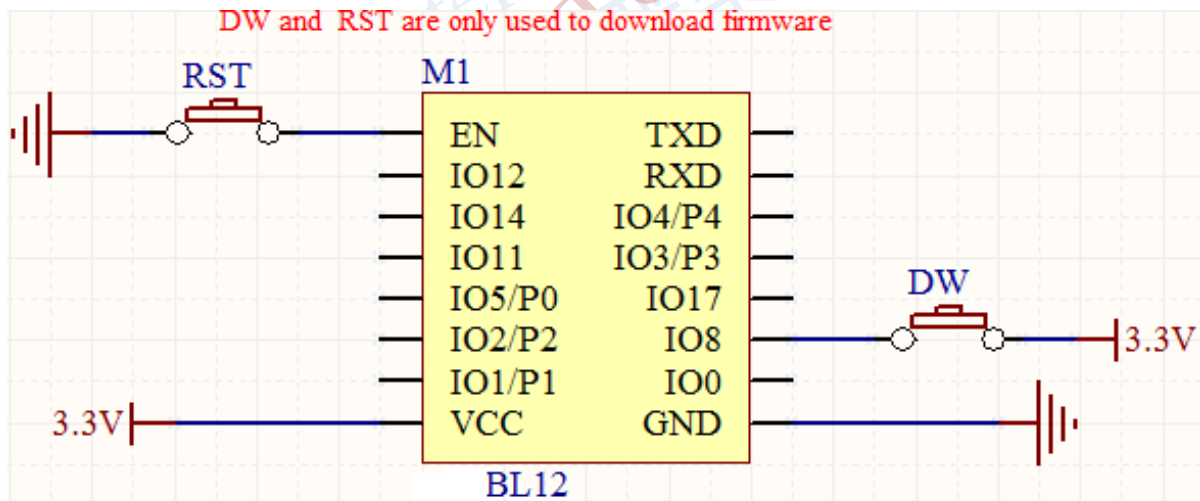
Fig.8.1 Minimum System
